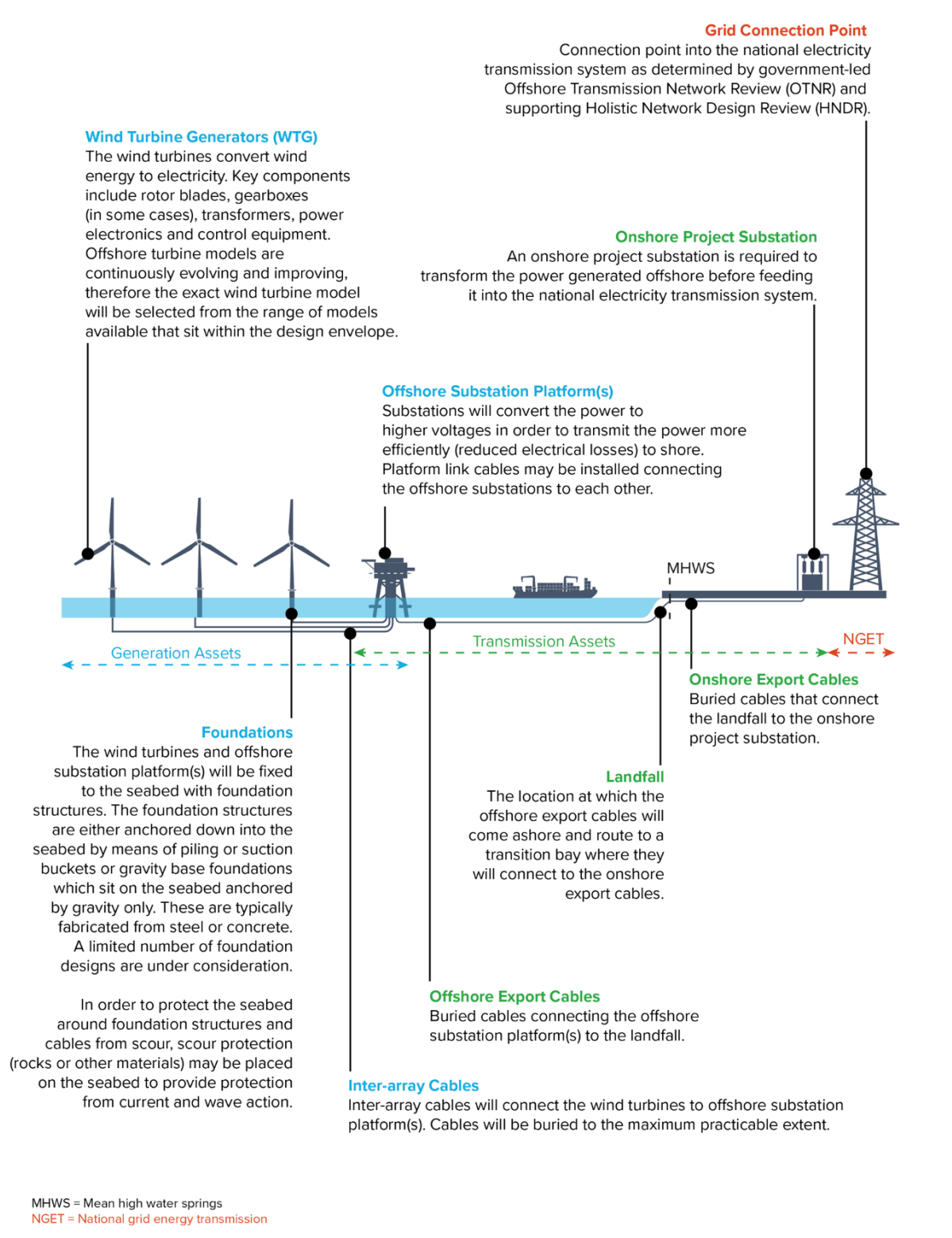
Plate 1.1 Components of Morecambe Offshore Windfarm Generation Assets ('the Project') are in blue. The components of Morgan and Morecambe Offshore Wind Farm: Transmission Assets ('Transmission Assets') are in green.
